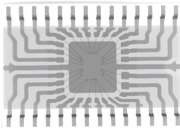
X-ray Image - 9751 date code
